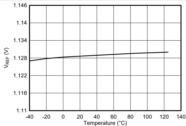
Figure 6-15. Reference Voltage vs Temperature ( V_{REF} = 1.129 V)
