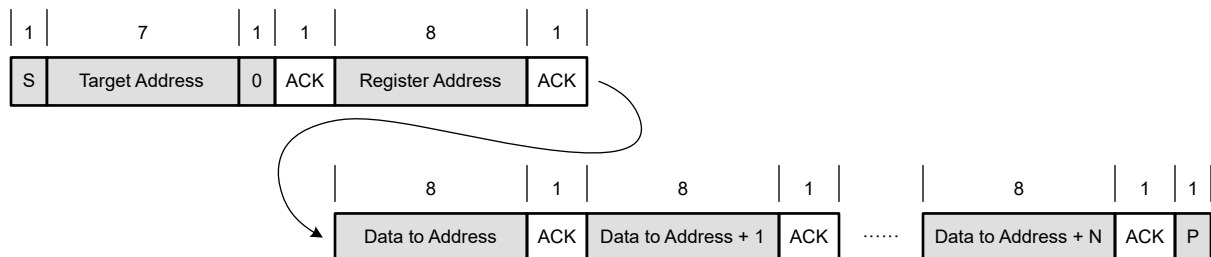
Figure 7-13. MultiByte Write
