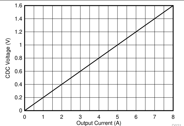
Figure 6-18. CDC Voltage vs Output Current with R SENSE = 10 mΩ
