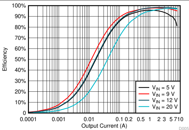
Figure 6-5. Efficiency vs Output Current, V_{OUT} = 12\text{ V} , FPWM
