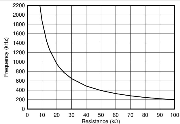
Figure 6-12. Switching Frequency vs Setting Resistance
