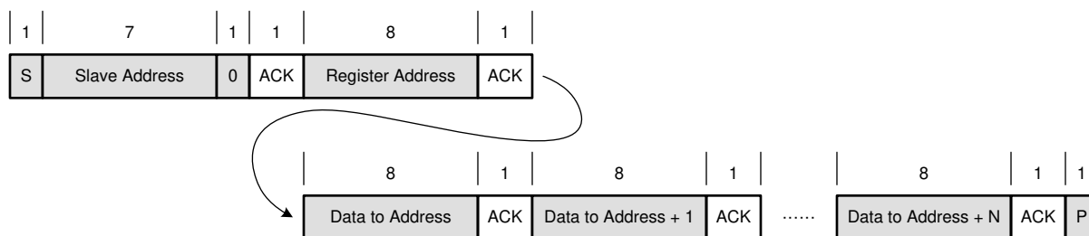
Figure 7-13. Multi-byte Write
