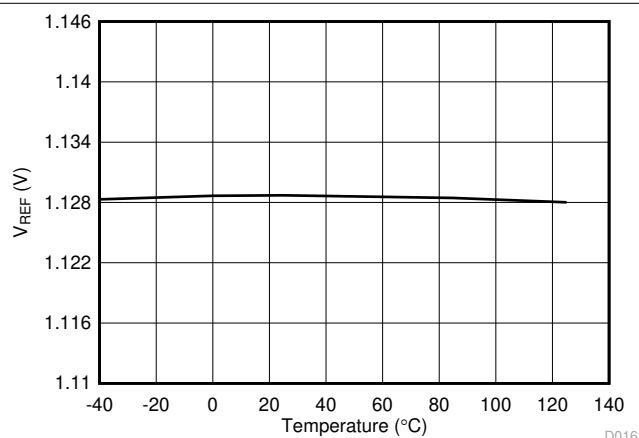
Figure 6-16. Reference Voltage vs Temperature (V REF = 1.129 V)
