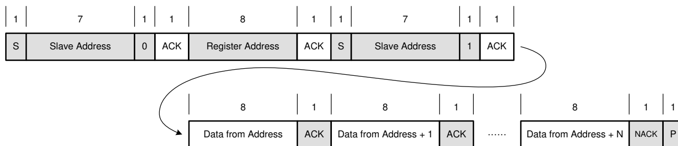
Figure 7-14. Multi-byte Read
