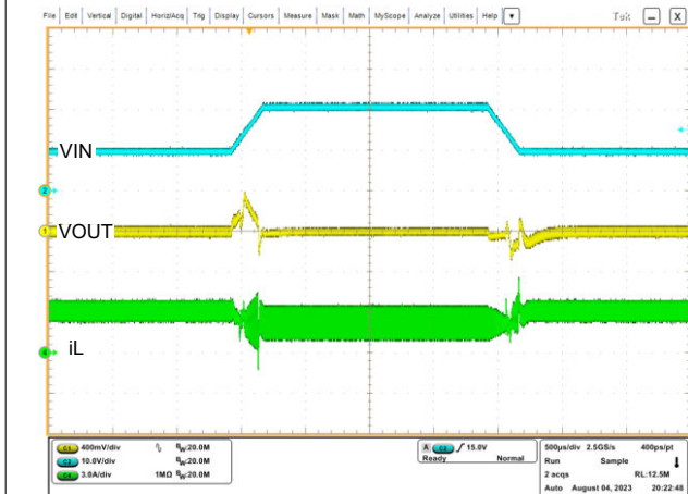
Figure 8-10. Line Transient Waveforms in V_{IN} = 9\text{ V} to 20\text{ V} , V_{OUT} = 12\text{ V} , I_O = 2\text{ A} with 200\text{-}\mu\text{s} Slew Rate, FPWM
