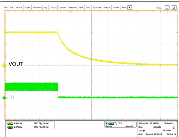
Figure 8-9. Shutdown Waveforms in V_{IN} = 16\text{ V} , V_{OUT} = 12\text{ V} , R_{LOAD} = 6\ \Omega , FPWM
