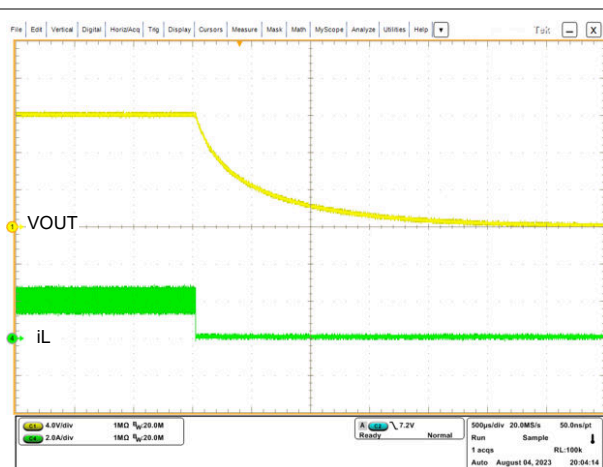
Figure 8-9. Shutdown Waveforms in V_{IN} = 16\text{ V} , V_{OUT} = 12\text{ V} , R_{LOAD} = 6\text{ }\Omega , FPWM
