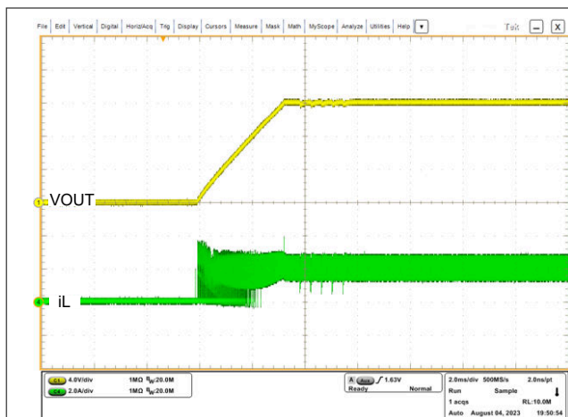
Figure 8-8. Start-up Waveforms in V_{IN} = 16\text{ V} , V_{OUT} = 12\text{ V} , R_{LOAD} = 6\text{ }\Omega , FPWM
