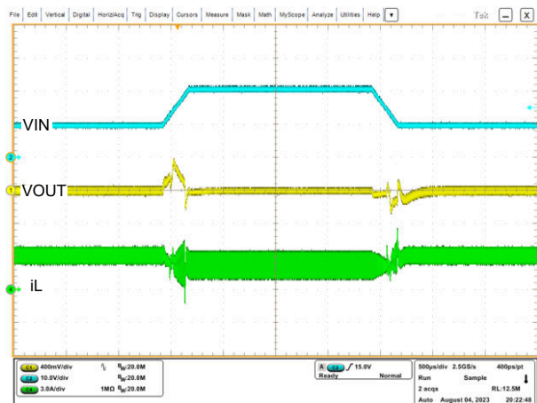
Figure 8-10. Line Transient Waveforms in V_{IN} = 9\text{ V} to 20\text{ V} , V_{OUT} = 12\text{ V} , I_O = 2\text{ A} with 200\text{-}\mu\text{s} Slew Rate, EPWM
