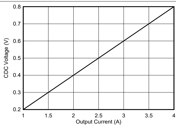
Figure 6-22. CDC Voltage vs Output Current with R_{\text{SENSE}} = 10 \text{ m}\Omega
