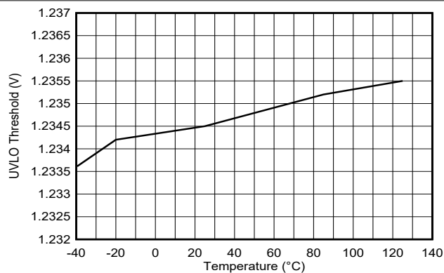
Figure 6-20. ENABLE/UVLO Rising Threshold vs Temperature
