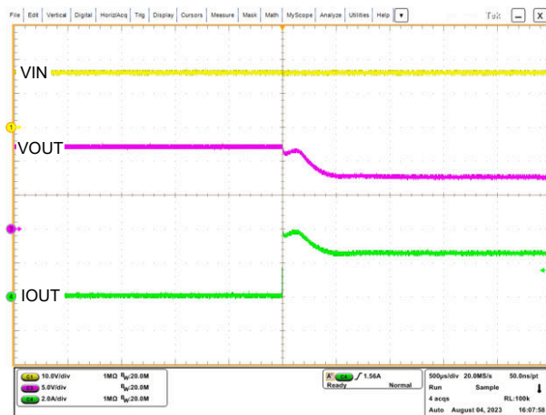
Figure 8-12. Output Current Limit Waveforms in V_{IN} = 16\text{ V} , V_{OUT} = 12\text{ V} , R_{LOAD} = 3\ \Omega , R_{SNS} = 20\text{ m}\Omega , FPWM
