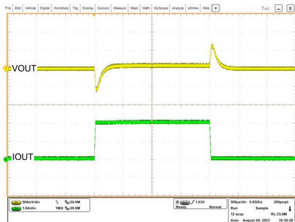
Figure 8-11. Load Transient Waveforms in V_{IN} = 16 V, V_{OUT} = 12 V, I_O = 0 A to 2 A with 20- \mu s Slew Rate, FPWM
