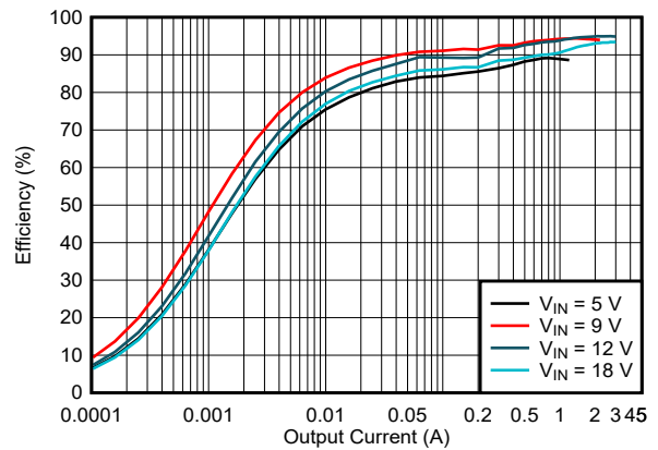
Figure 5-14. Efficiency vs Output Current, V_{OUT} = 12V , f_{SW} = 2\text{ MHz} , PFM
