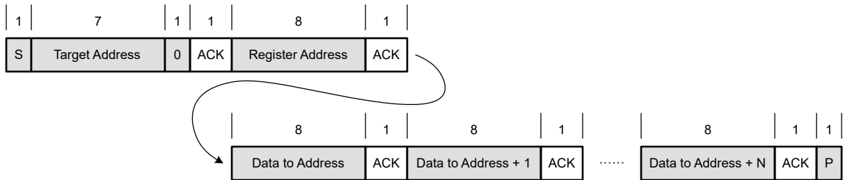
Figure 6-13. Multi-byte Write
