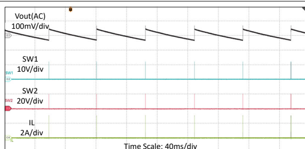
Figure 8-7. Switching Waveforms in V_{IN} = 12V , V_{OUT} = 20V , I_O = 0A , PFM
