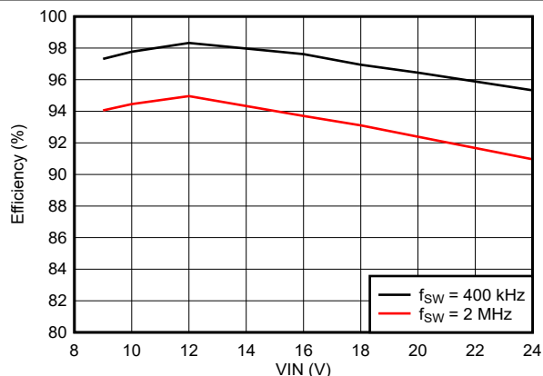
Figure 5-15. Efficiency vs Input Voltage, V OUT = 12 V, I OUT = 2A, FPWM
