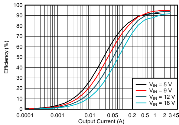
Figure 5-11. Efficiency vs Output Current, V_{OUT} = 9V , f_{SW} = 2\text{ MHz} , FPWM
