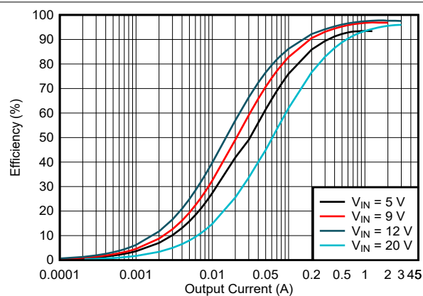
Figure 5-5. Efficiency vs Output Current, V_{OUT} = 12V , f_{SW} = 400\text{ kHz} , FPWM
