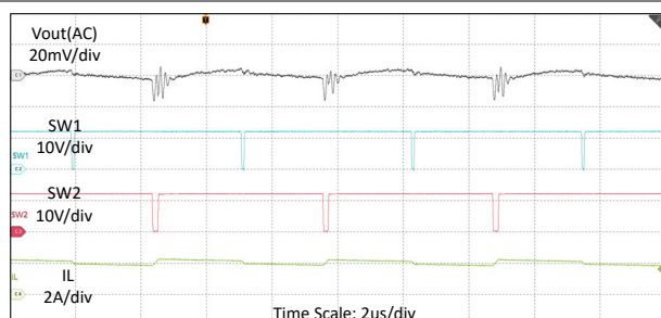
Figure 8-4. Switching Waveforms in V_{IN} = 12V , V_{OUT} = 12V , I_O = 2A , FPWM
