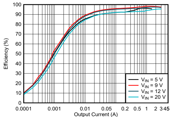
Figure 5-4. Efficiency vs Output Current, V_{OUT} = 9V , f_{SW} = 400\text{ kHz} , PFM
