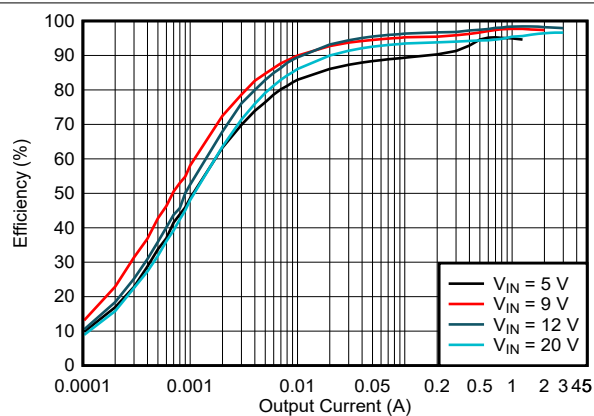
Figure 5-6. Efficiency vs Output Current, V_{OUT} = 12V , f_{SW} = 400\text{ kHz} , PFM
