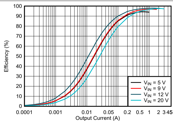
Figure 5-7. Efficiency vs Output Current, V_{OUT} = 15V , f_{SW} = 400\text{ kHz} , FPWM
