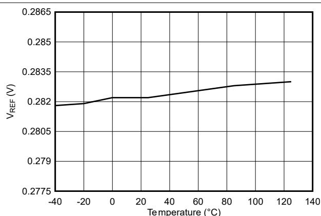
Figure 5-17. Reference Voltage vs Temperature (V REF = 0.282V)
