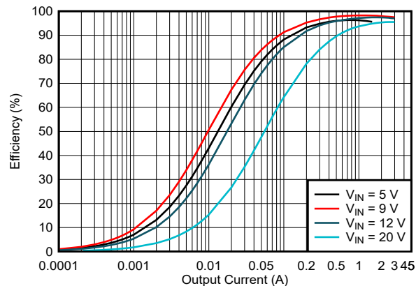
Figure 5-3. Efficiency vs Output Current, V_{OUT} = 9V , f_{SW} = 400\text{ kHz} , FPWM
