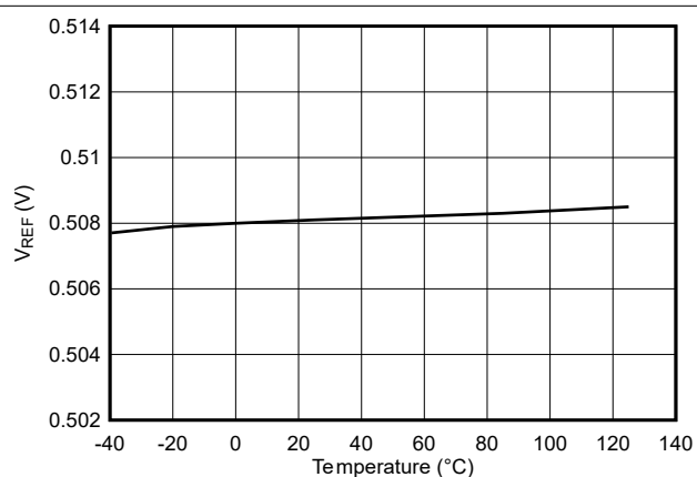
Figure 5-18. Reference Voltage vs Temperature (V REF = 0.508V)
