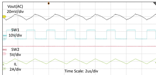
Figure 8-2. Switching Waveforms in V_{IN} = 12V , V_{OUT} = 5V , I_O = 2A , FPWM
