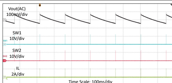
Figure 8-5. Switching Waveforms in V_{IN} = 12V , V_{OUT} = 12V , I_O = 0A , PFM
