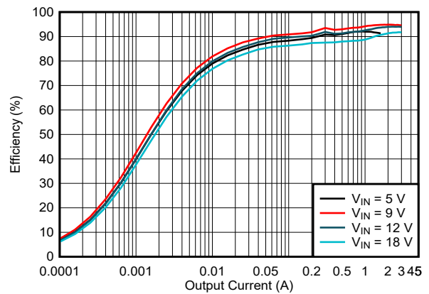
Figure 5-12. Efficiency vs Output Current, V_{OUT} = 9V , f_{SW} = 2\text{ MHz} , PFM
