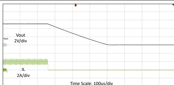
Figure 8-9. Shutdown Waveforms in V_{IN} = 12V , V_{OUT} = 5V , R_{LOAD} = 2.5\Omega , FPWM
