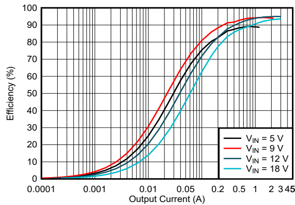
Figure 5-13. Efficiency vs Output Current, V_{OUT} = 12V , f_{SW} = 2\text{ MHz} , FPWM
