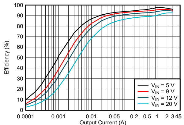
Figure 5-2. Efficiency vs Output Current, V_{OUT} = 5\text{ V} , f_{sw} = 400\text{ kHz} , PFM
