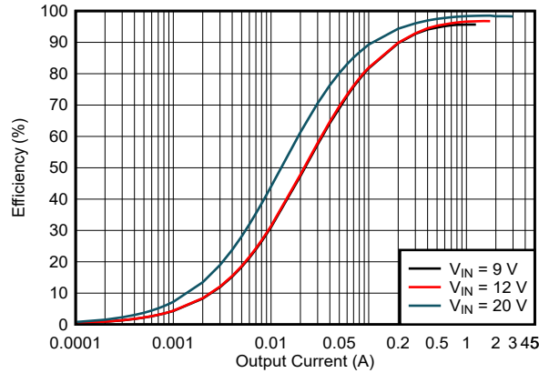
Figure 5-9. Efficiency vs Output Current, V_{OUT} = 20V , f_{SW} = 400\text{ kHz} , FPWM
