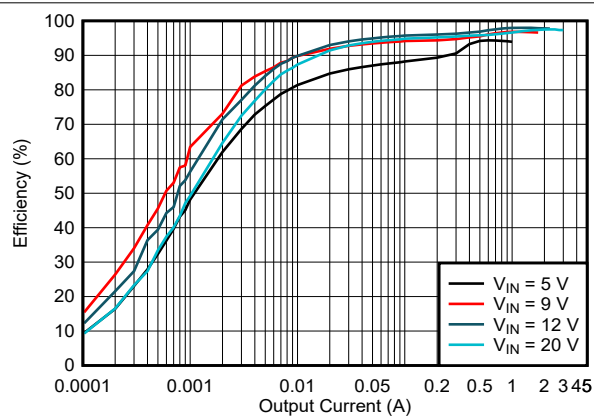
Figure 5-8. Efficiency vs Output Current, V_{OUT} = 15V , f_{SW} = 400\text{ kHz} , PFM
