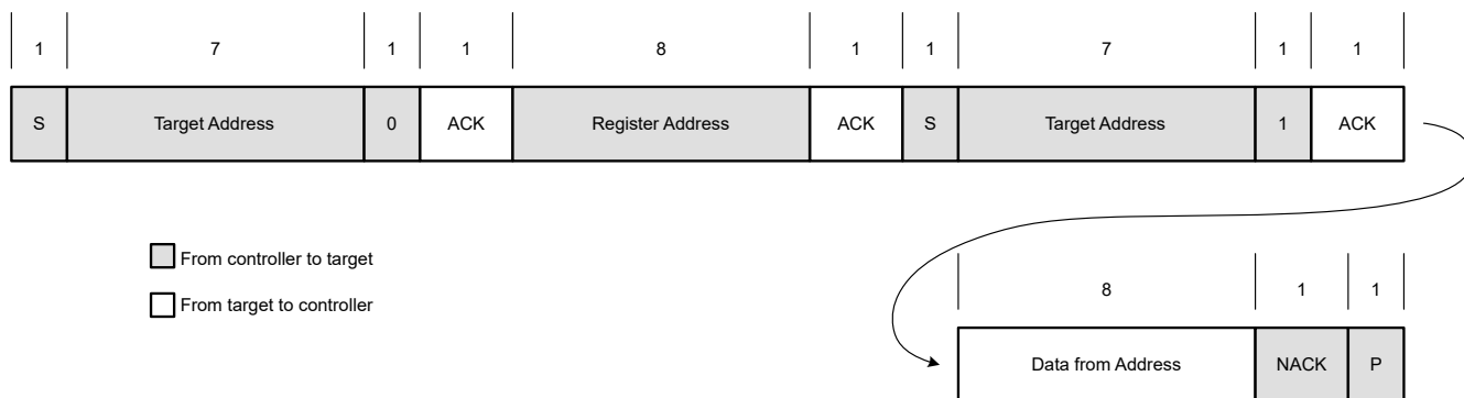
Figure 6-12. Single-Byte Read
