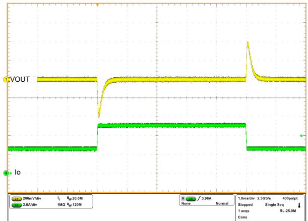
Figure 7-11. Load Transient Waveforms in V_{IN} = 12V , V_{OUT} = 5V , I_O = 2.5A to 5A with 20\mu s Slew Rate, FPWM
