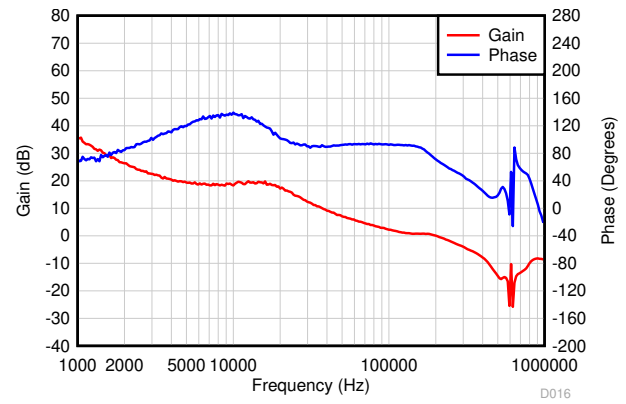
Figure 6-20. Frequency Response, 20 A Load
