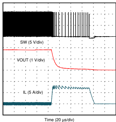
Figure 7-28. Overcurrent Response
