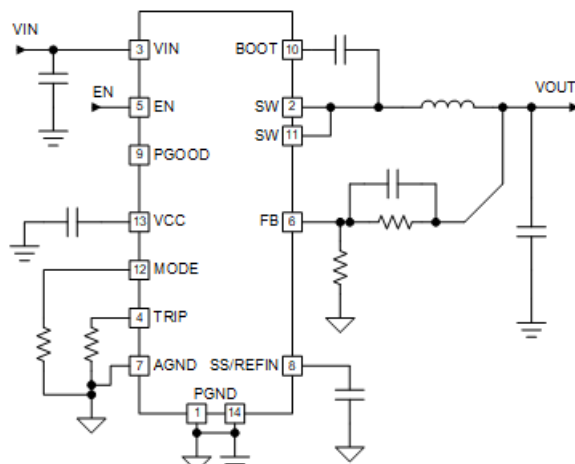
Simplified Schematic
