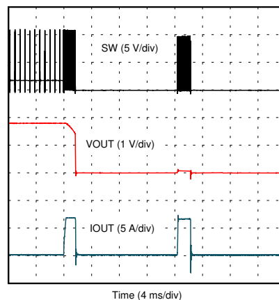
Figure 7-29. Overcurrent Response
