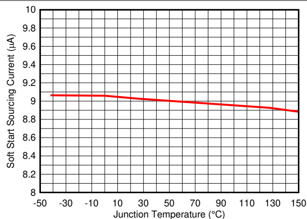
Figure 5-12. Soft-Start Sourcing Current
