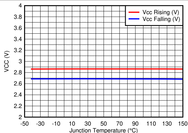
Figure 5-8. VCC UVLO
