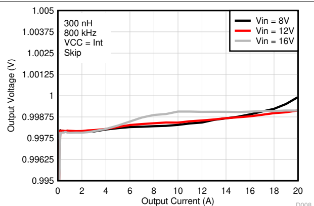
Figure 8-7. Output Voltage vs Output Current
