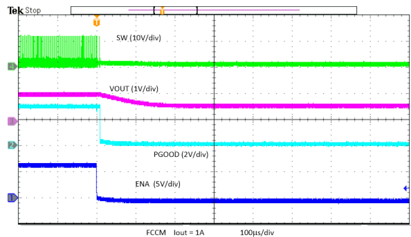
Figure 8-15. Prebias Power-Down
