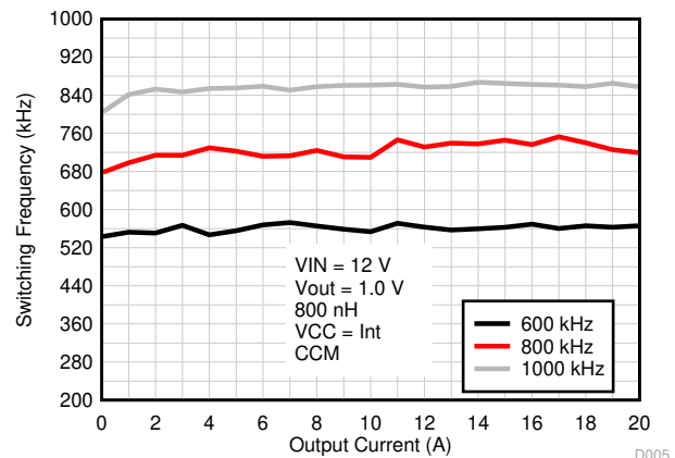
Figure 8-5. Switching Frequency vs Output Current
