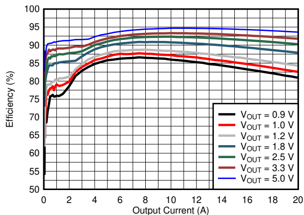
Efficiency Graph, 12 V IN , 800 kHz, DCM, Internal V CC
