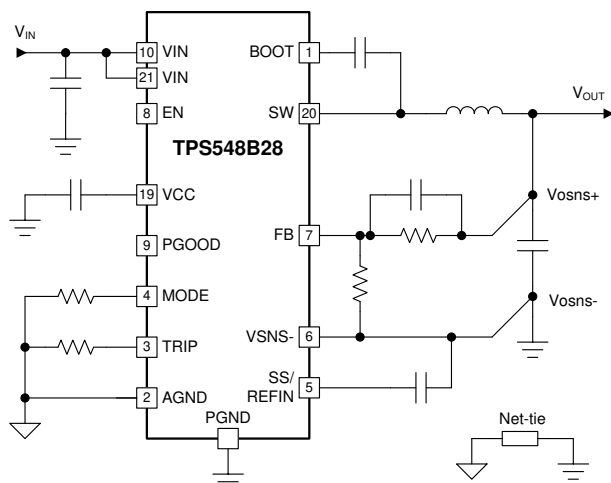
Simplified Schematic
