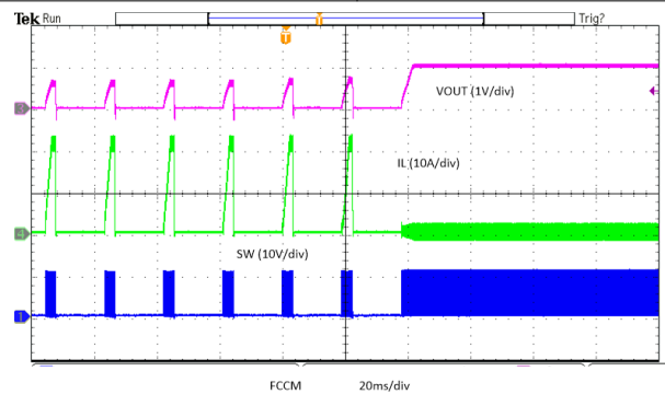
Figure 8-30. Hiccup Overcurrent
