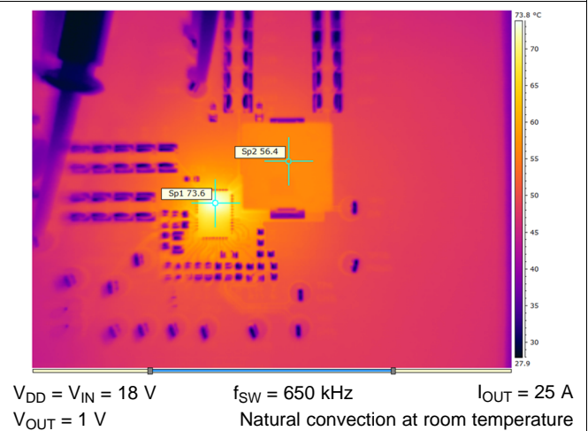
Figure 10. Thermal Image
