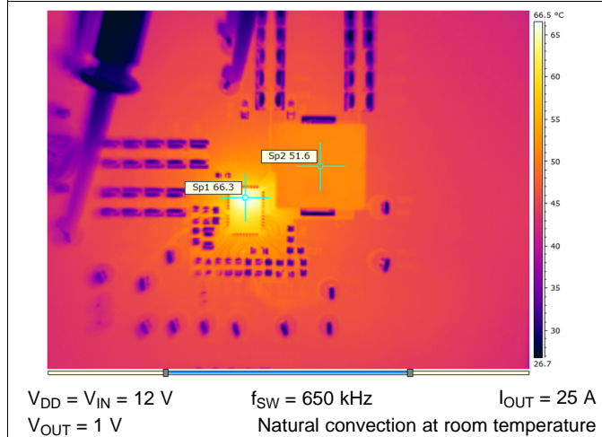
Figure 9. Thermal Image
