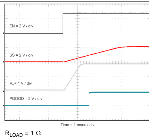
Figure 44. EN Startup
