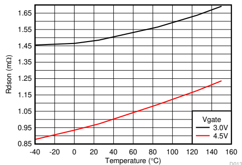
Figure 6-13. Low-Side MOSFET On-Resistance ( R_{DS(on)} ) vs Junction Temperature
