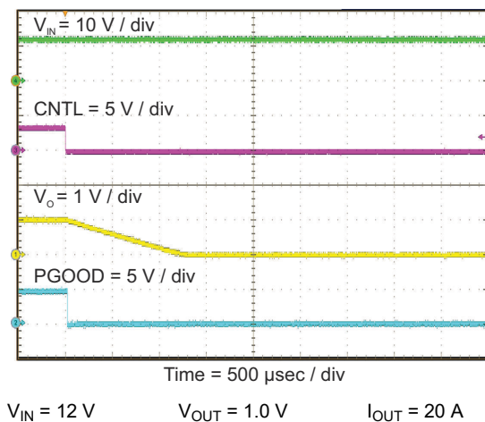
Figure 8-6. Shutdown from CNTL
