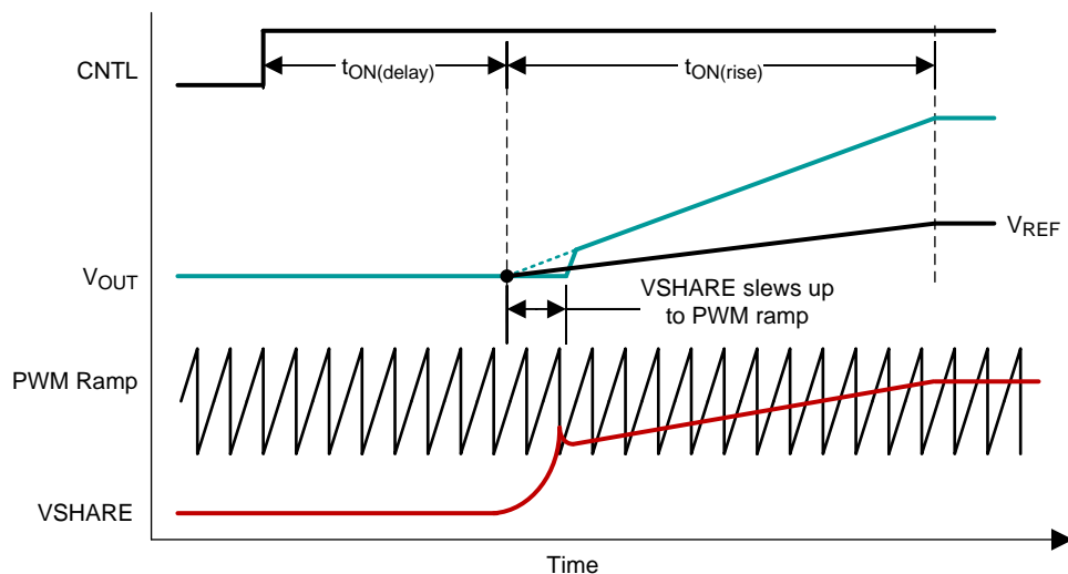
Figure 31. Soft-Start Timing
