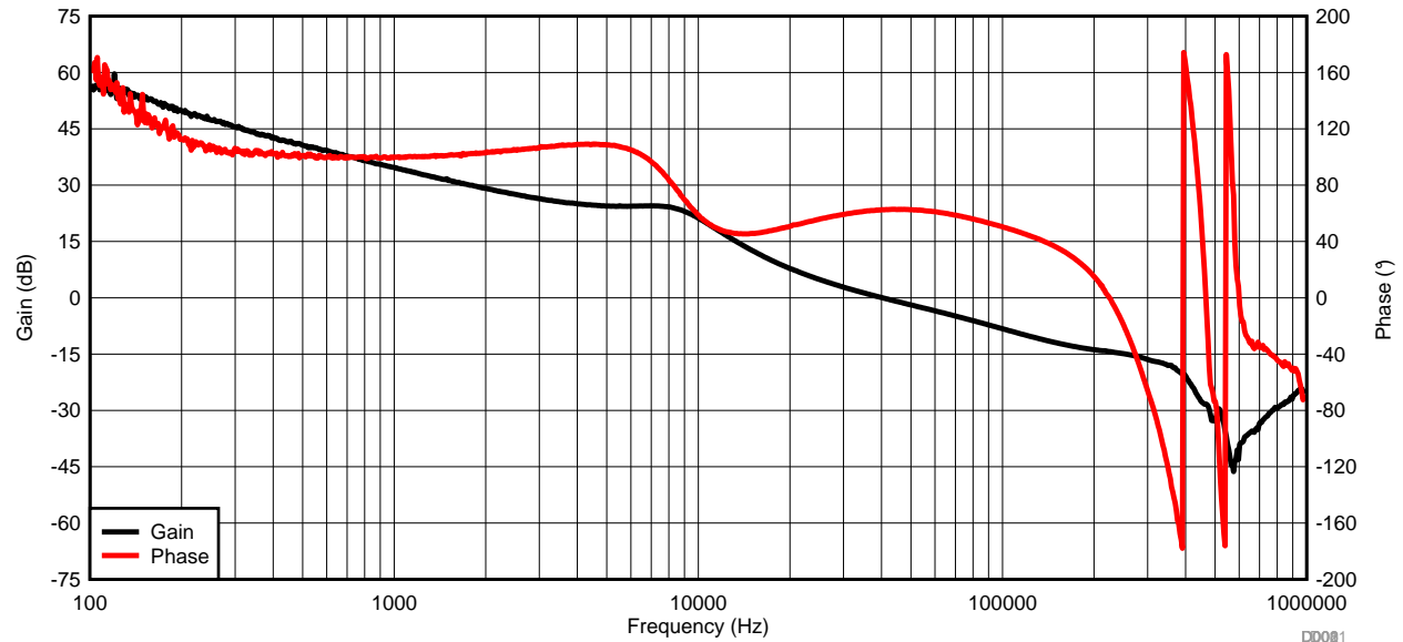
Figure 45. Total-Loop Bode Plot
