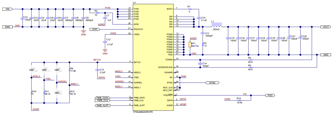
Figure 7-1. TPS546B24S Application
