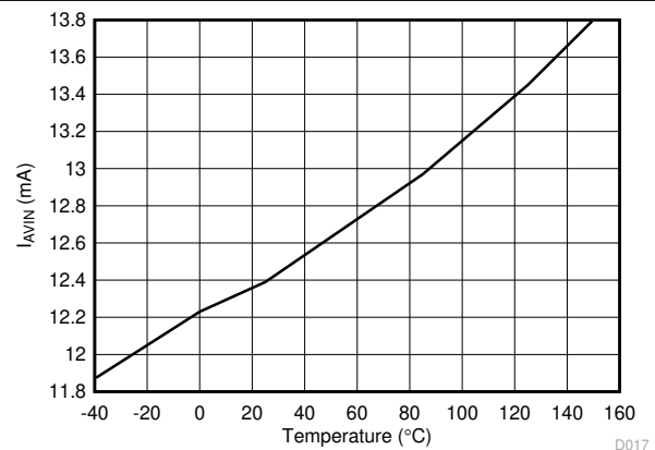
Figure 6-10. Non-Switching Input Current ( I_{AVIN} ) vs Junction Temperature
