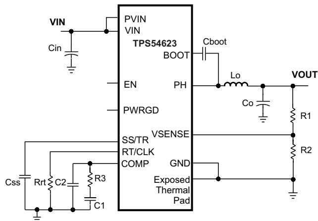
Simplified Schematic
