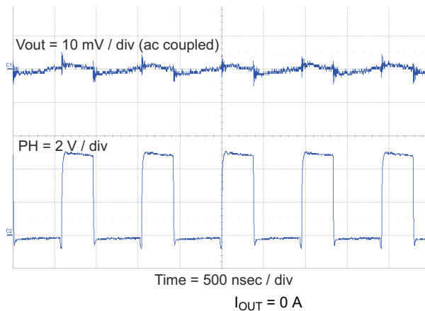
Figure 8-7. Output Ripple
