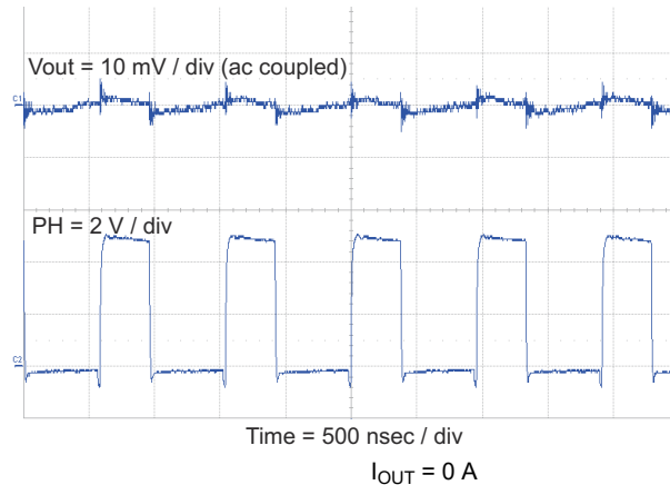
Figure 8-7. Output Ripple
