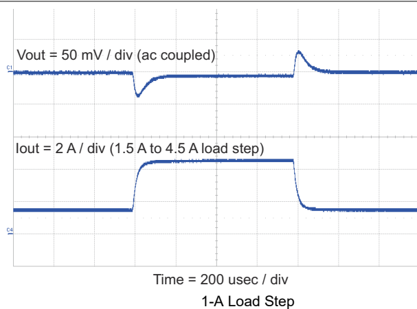
Figure 8-4. Transient Response
