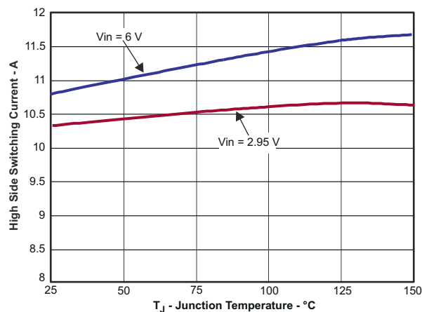
Figure 6-3. High-Side Current Limit vs Junction Temperature
