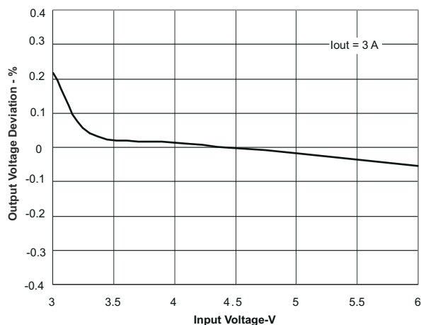
Figure 8-11. Regulation vs Input Voltage
