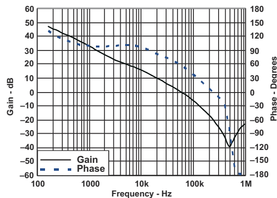
Figure 8-9. Closed-Loop Response
