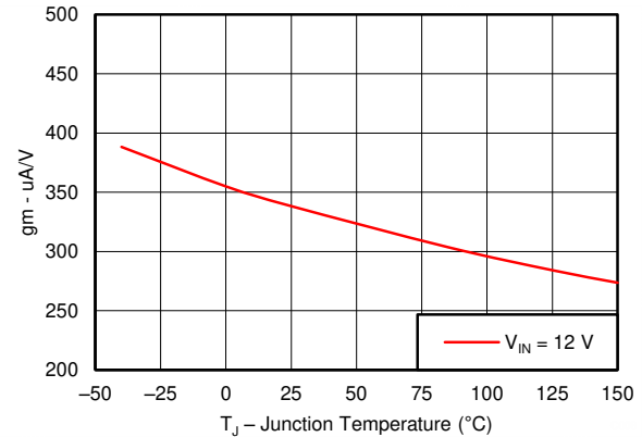
Figure 6-8. EA Transconductance vs Junction Temperature
