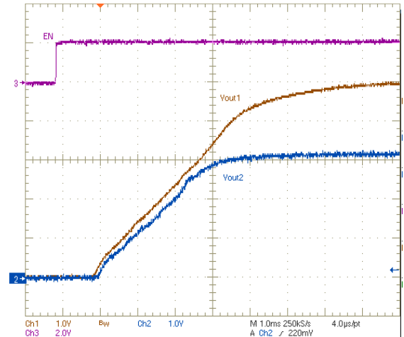
Figure 7-10. Ratio-Metric Startup with Tracking Resistors
