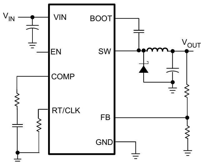
Simplified Schematic
