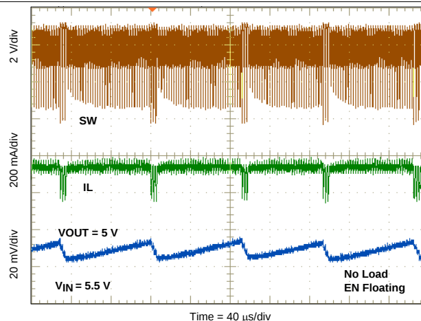
Figure 46. Low Dropout Operation
