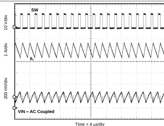
Figure 44. Input Ripple CCM
