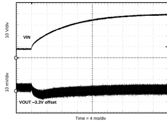
Figure 38. Line Transient (8 V to 40 V)
