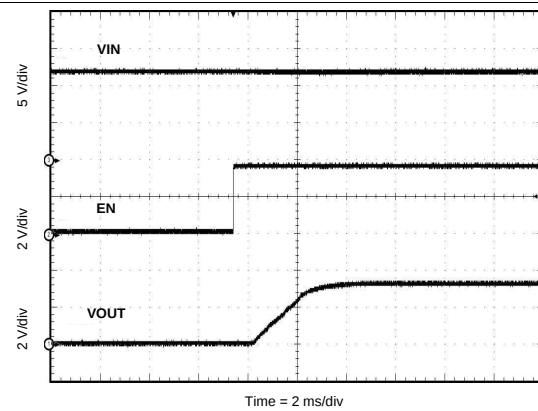
Figure 40. Start-up With EN
