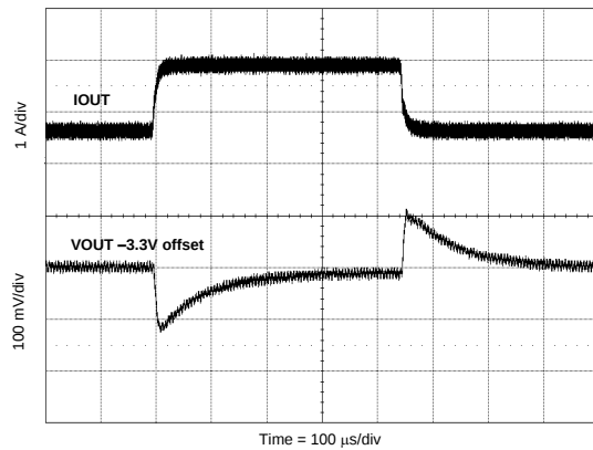
Figure 37. Load Transient
