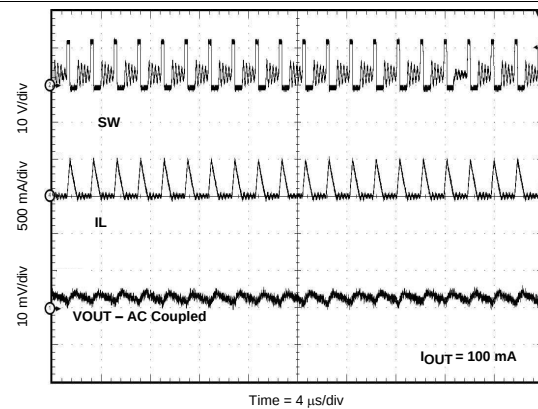
Figure 42. Output Ripple DCM
