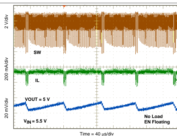
Figure 45. Low Dropout Operation
