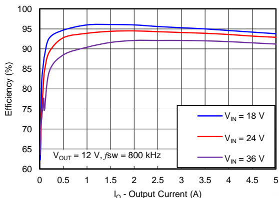
Figure 50. Efficiency vs Output Current
