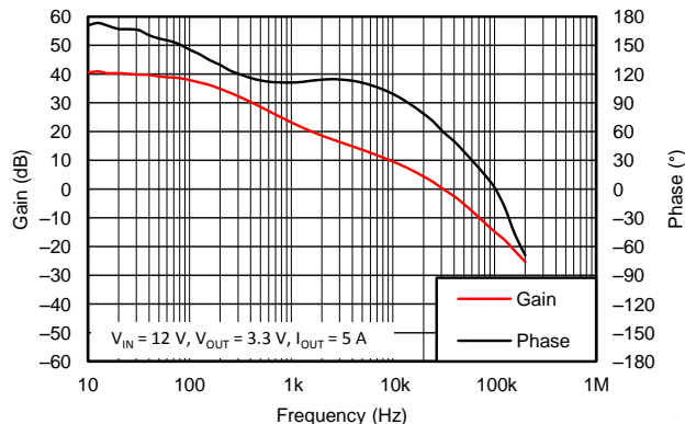
Figure 51. Overall Loop Frequency Response
