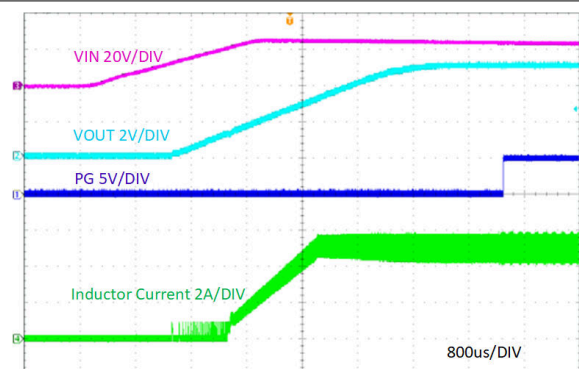
Figure 7-10. Start-Up Relative to V_{IN} , I_{OUT} = 5A
