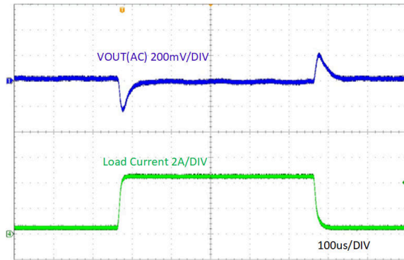
Figure 7-14. Load Transient Response, 0.5 to 4.5A, Slew Rate = 0.8A/μS
