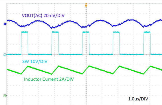
Figure 7-13. Steady State, I_{OUT} = 5A
