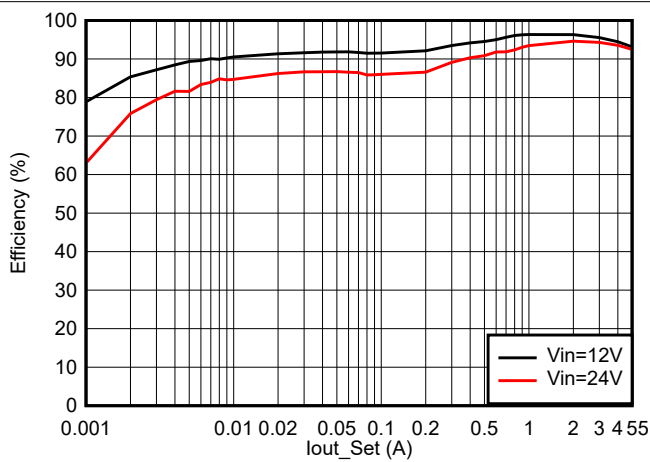
Figure 7-2. Efficiency (PFM)
