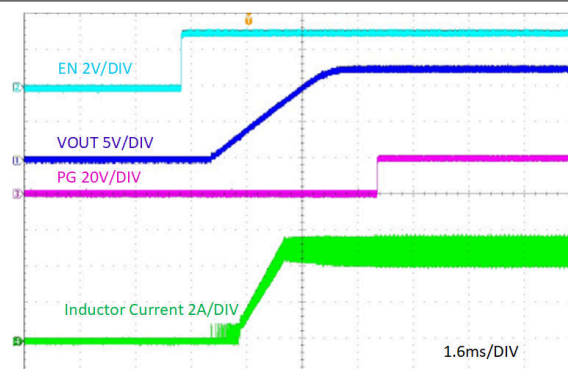
Figure 7-11. Start-Up Through EN, I_{OUT} = 5A
