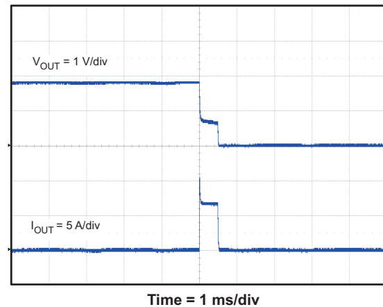
Figure 51. Hiccup Mode Current Limit
