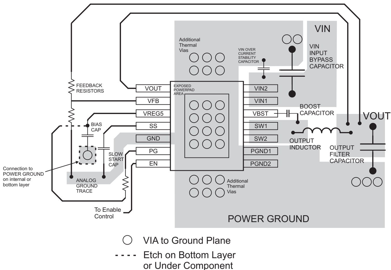
Figure 16. PCB Layout
