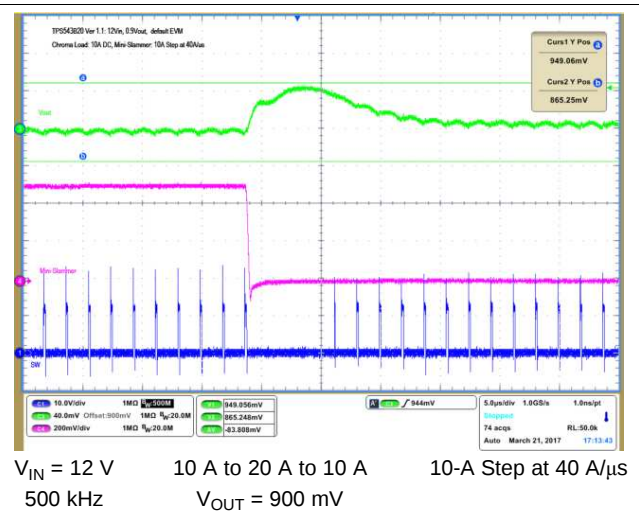
Figure 26. Transient Response When Load Steps Down
