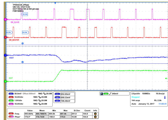
Figure 30. Transient Response of 25-A to 50-A Load at 30 A/ \mu s Rise
