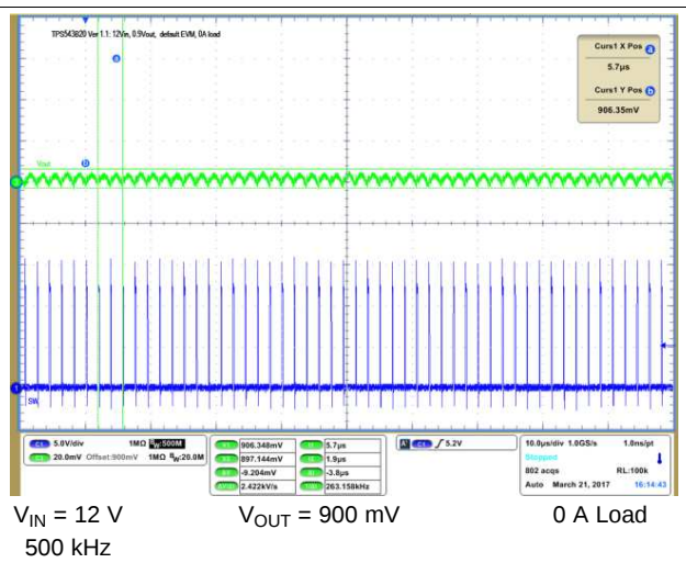
Figure 8. Output Voltage Ripple at Steady State
