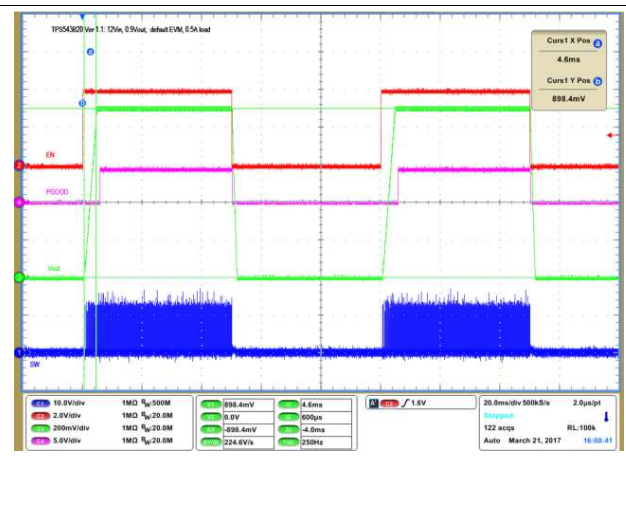
Figure 12. Output Voltage Start-Up and Shutdown
