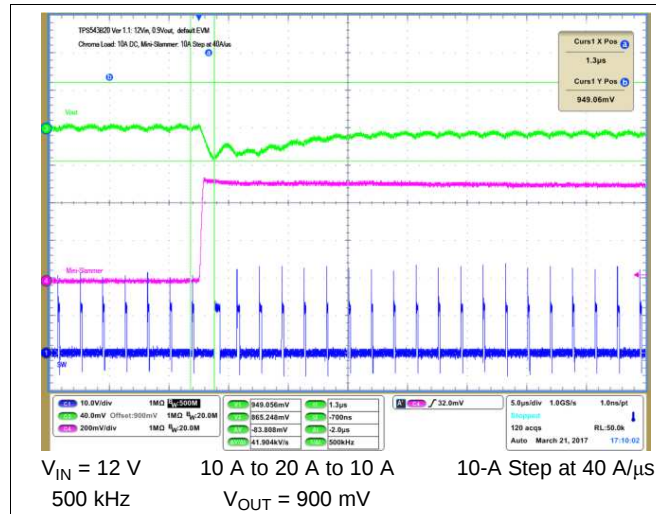
Figure 25. Transient Response When Load Steps Up
