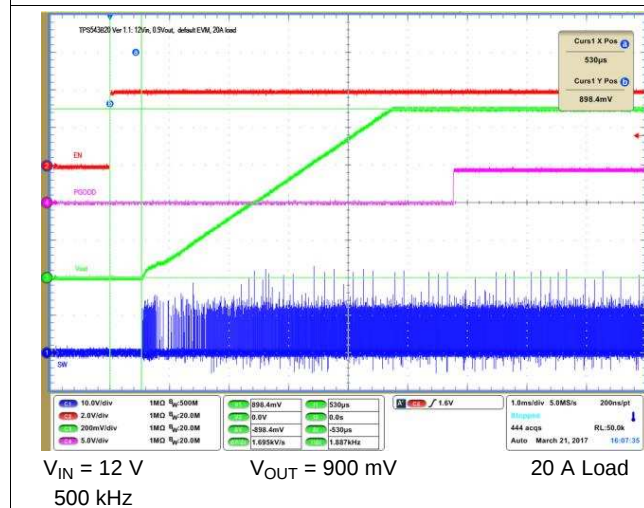
Figure 11. Start-Up From EN
