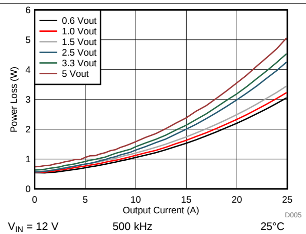
Figure 4. Power Loss vs Output Current
