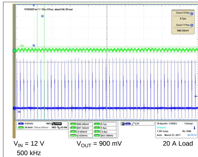
Figure 9. Output Voltage Ripple at Steady State
