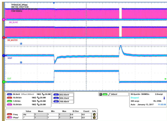
Figure 29. Transient Response of 0.9-V Output at 12 V_{IN} , Transient is 25 A to 50 A, Step is 25 A at 30 A/ \mu s
