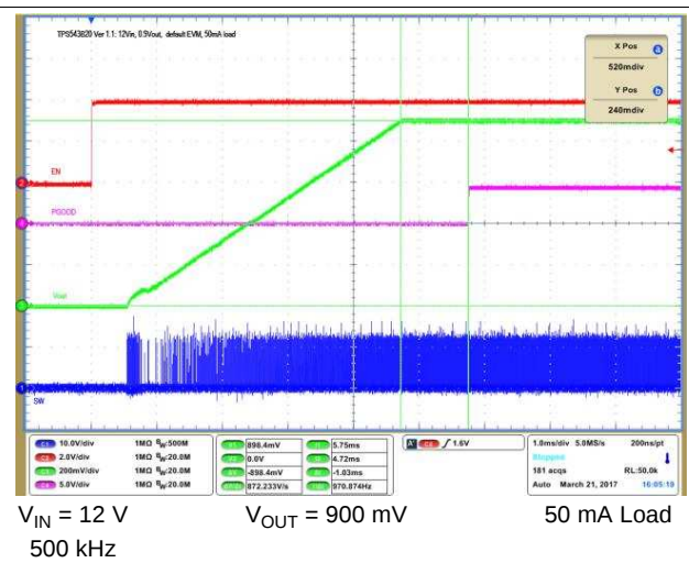
Figure 10. Startup From EN
