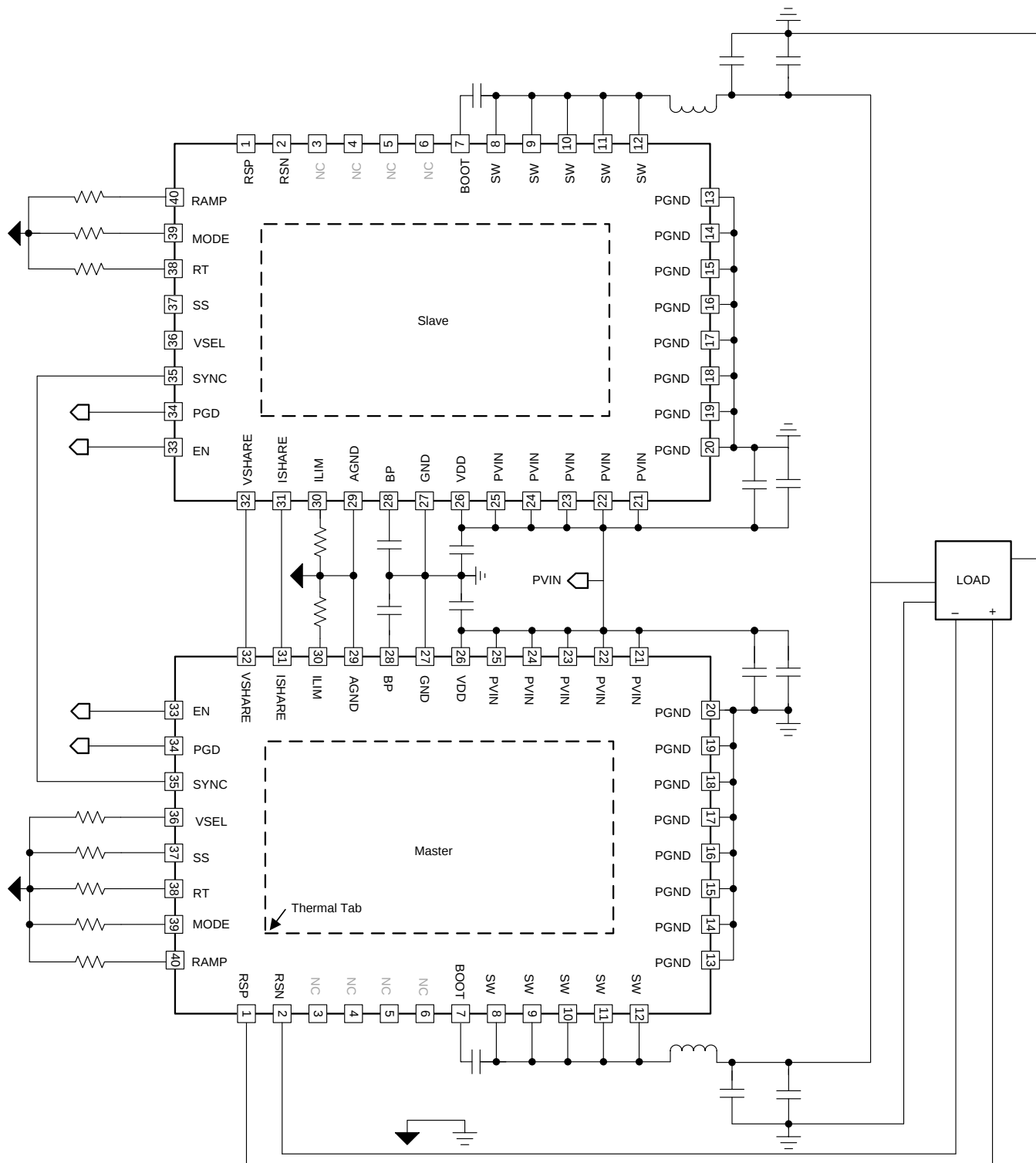
Figure 28. 2-Phase Stackable
