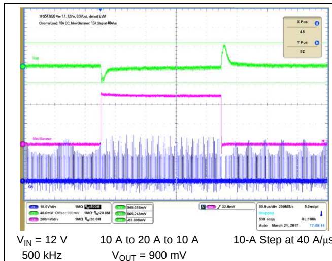
Figure 7. Output Voltage Transient Response
