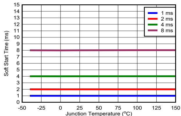
Figure 5-12. Soft Start
