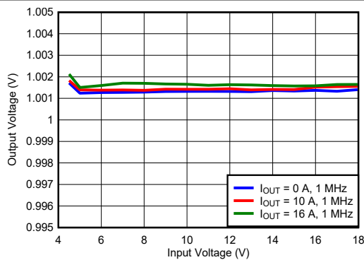
Figure 7-6. Line Regulation
