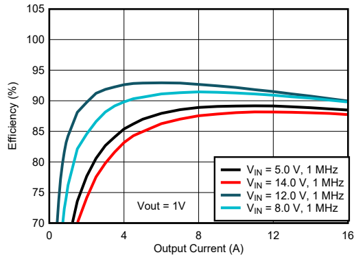
Figure 7-4. Efficiency Curves
