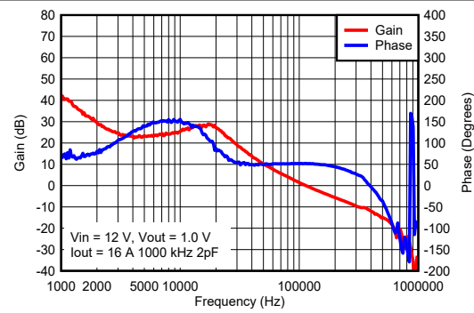
Figure 7-7. Bode Plot
