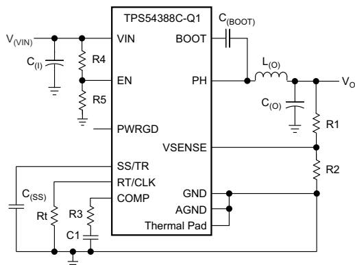
Simplified Schematic
