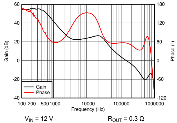
Figure 8-7. Bode Plot
