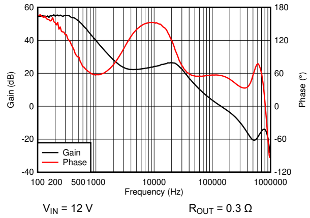
Figure 8-7. Bode Plot
