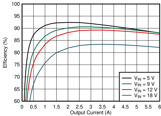
Figure 8-4. Efficiency
