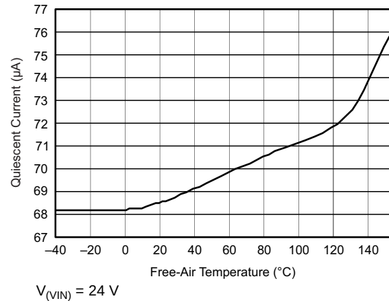
Figure 7. LPM, Quiescent Current Variation with Temperature
