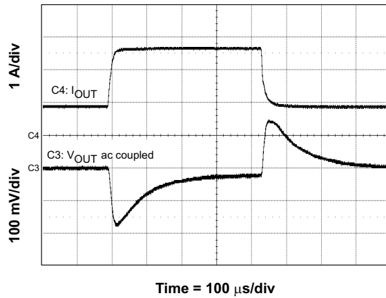
Figure 33. Load Transient
