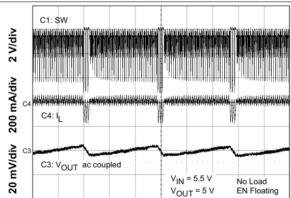
Time = 20 \mu s/div Figure 44. Low Dropout Operation
