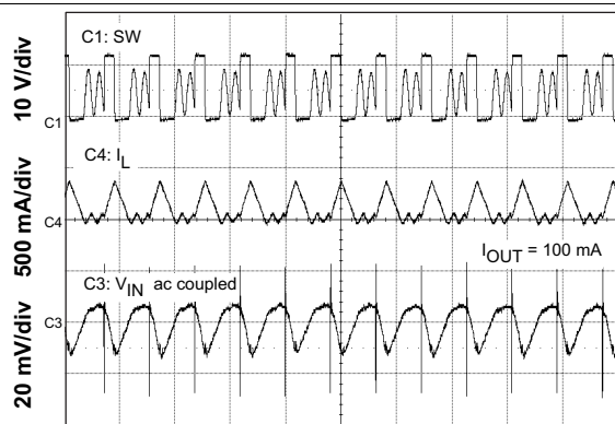
Time = 2 \mu s/div Figure 43. Input Ripple DCM
