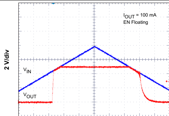
Time = 40 \mu s/div Figure 45. Low Dropout Operation
