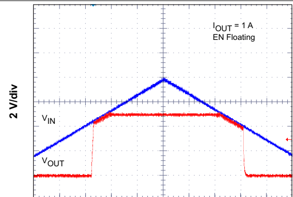
Time = 40 \mu s/div Figure 46. Low Dropout Operation
