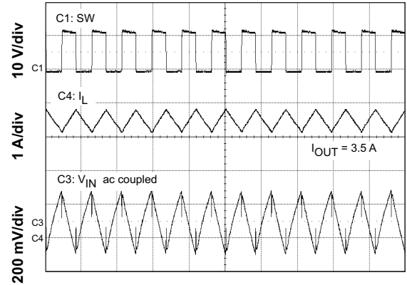
Time = 2 \mu s/div Figure 42. Input Ripple CCM
