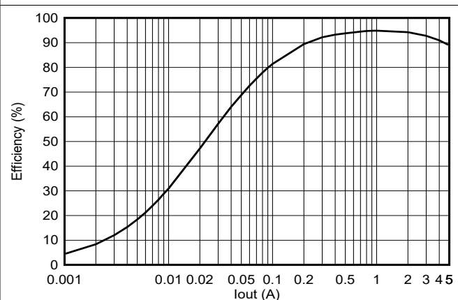
Figure 5-16. TPS543521 Efficiency (FCCM), V_{IN} = 12\text{V} , V_{OUT} = 3.3\text{V} , f_{SW} = 500\text{kHz} , L = 4.7\mu\text{H}
