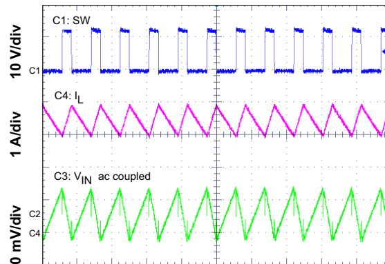
Time = 2 μs/div I_{OUT} = 3.5 \text{ A}
