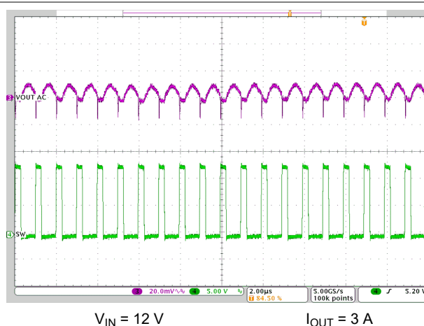
V_{IN} = 12\text{ V} I_{OUT} = 3\text{ A} Figure 8-15. Output Ripple – 3-A Load
