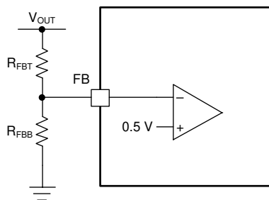
Figure 7-3. FB Resistor Divider
