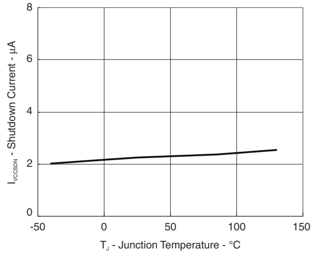
Figure 6-2. V_{CC} Shutdown Current vs Junction Temperature
