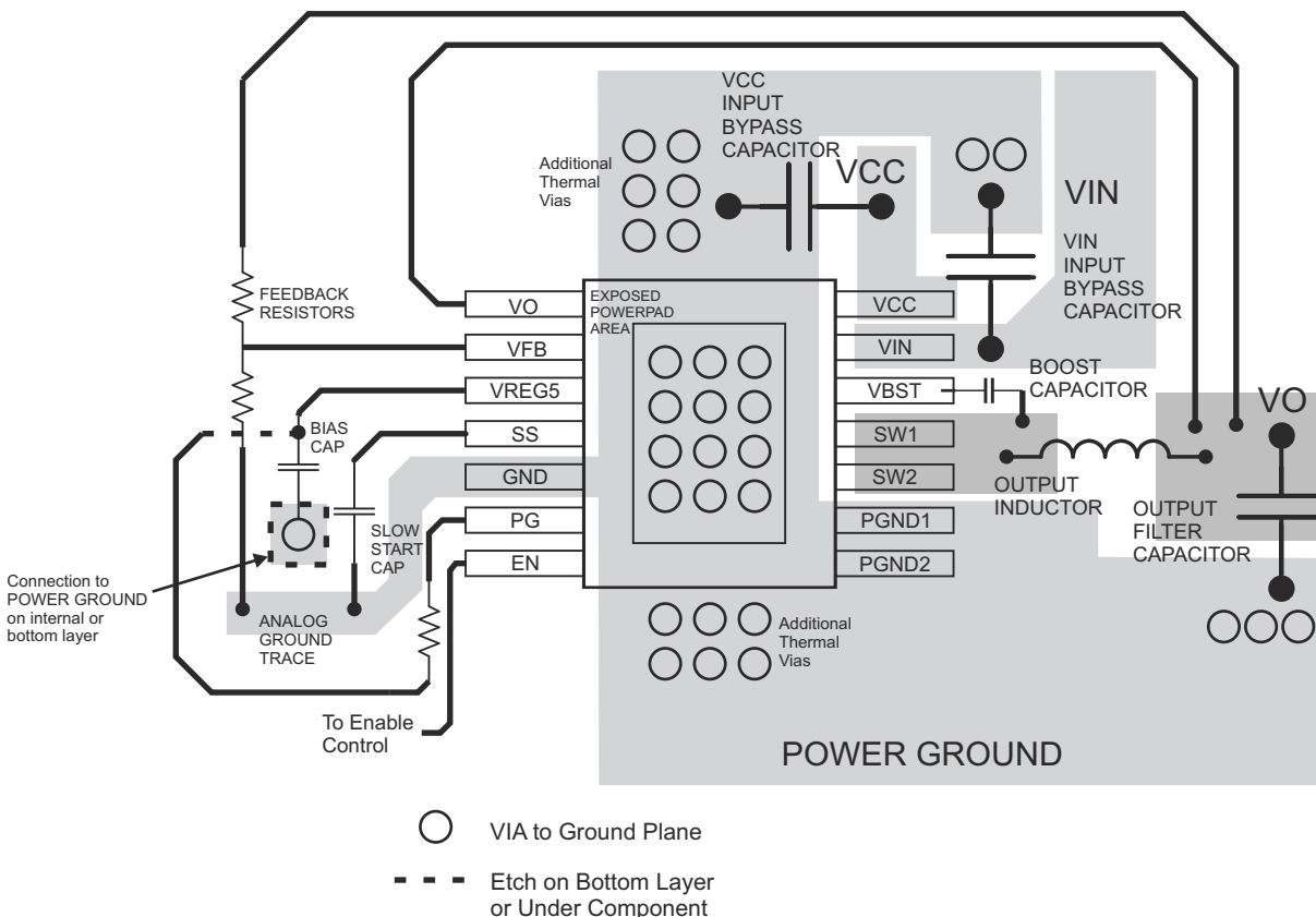
Figure 10-1. PCB Layout
