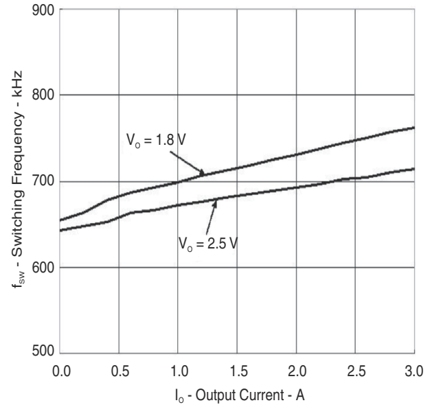
Figure 6-4. Switching Frequency vs Output Current
