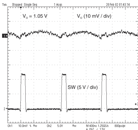
Figure 8-6. Voltage Ripple at Output
