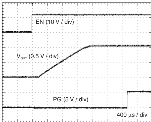
Figure 8-4. Start-Up Waveform
