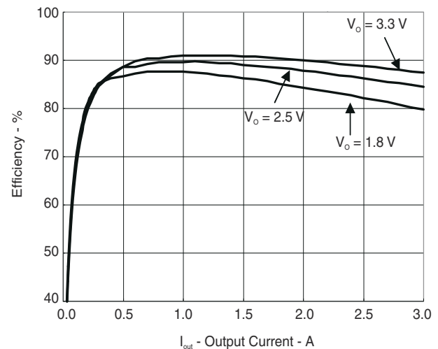
Figure 8-5. Efficiency vs Output Current ( V_{IN} = 12\text{ V} )
