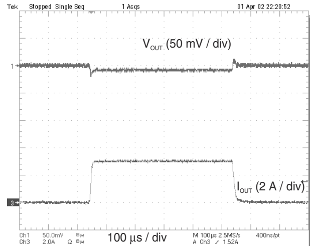
Figure 8-3. 1.05-V, 0-A to 3-A Load Transient Response
