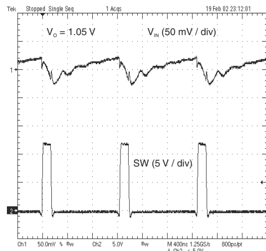
Figure 8-7. Voltage Ripple at Input
