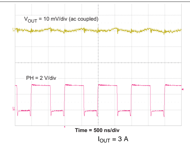
Figure 49. Input Ripple
