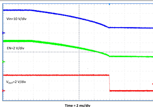
Figure 8-13. Shutdown Relative to VIN
