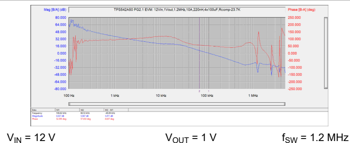
V_{IN} = 12\text{ V} V_{OUT} = 1\text{ V} f_{SW} = 1.2\text{ MHz} Figure 8-4. Bode Plot at 10-A Output Current
