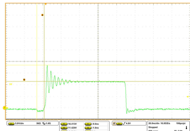
Figure 6-22. Switch Node Ringing and Dead-Time at 10-A Output Current
