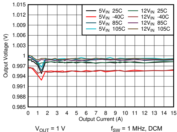
Figure 6-8. Load Regulation
