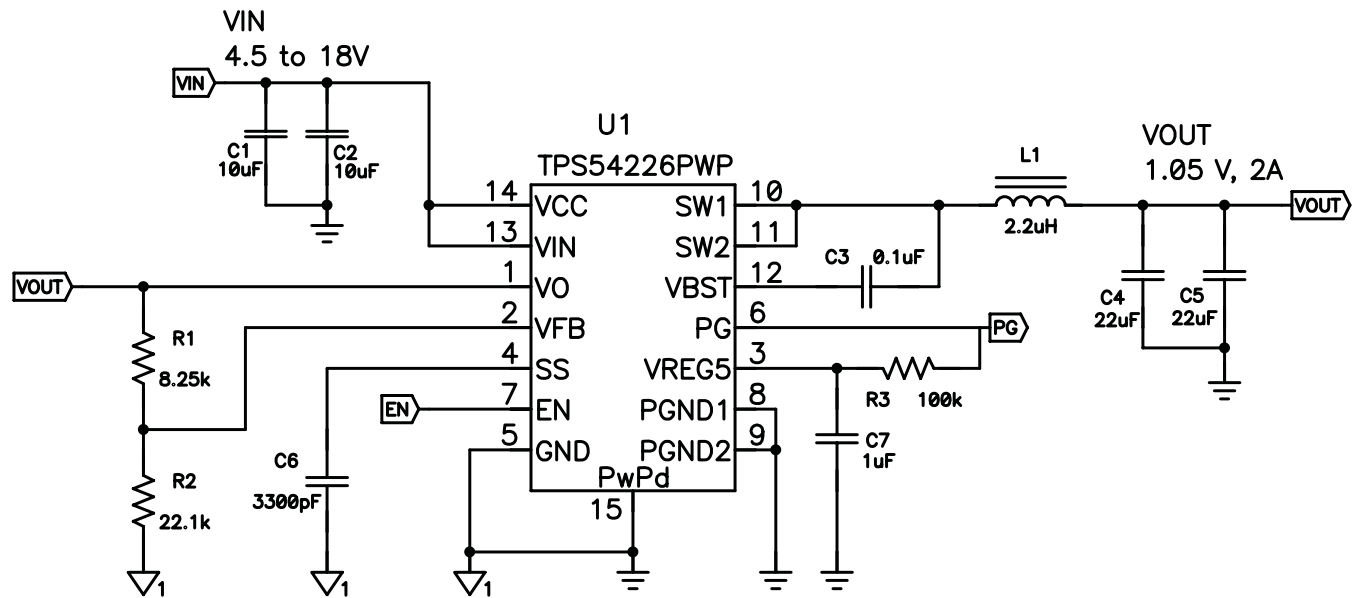
Figure 14. Schematic Diagram
