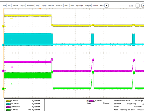
CH1: V_{OUT} CH2: SW CH3: FB CH4: Inductor current
