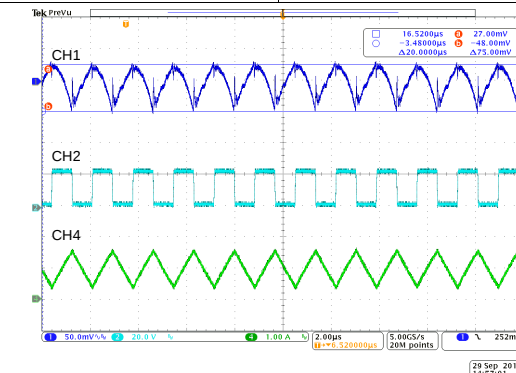
CH1: V_{VIN} (AC-coupled) CH2: SW CH4: Inductor current
