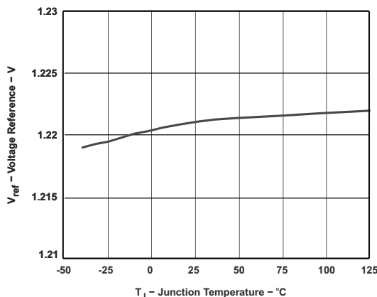
Figure 7-4. VOLTAGE REFERENCE vs JUNCTION TEMPERATURE
