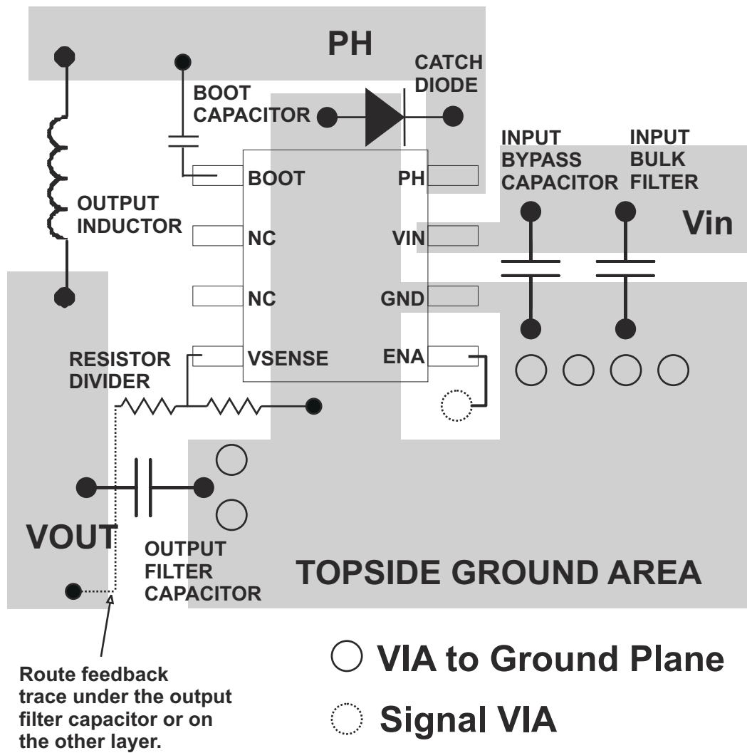
Figure 8-1. Design Layout
