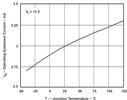
Figure 7-2. OPERATING QUIESCENT CURRENT vs JUNCTION TEMPERATURE
