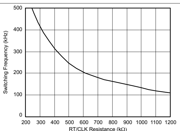
Figure 42. Switching Frequency vs RT/CLK Resistance Low Frequency Range
