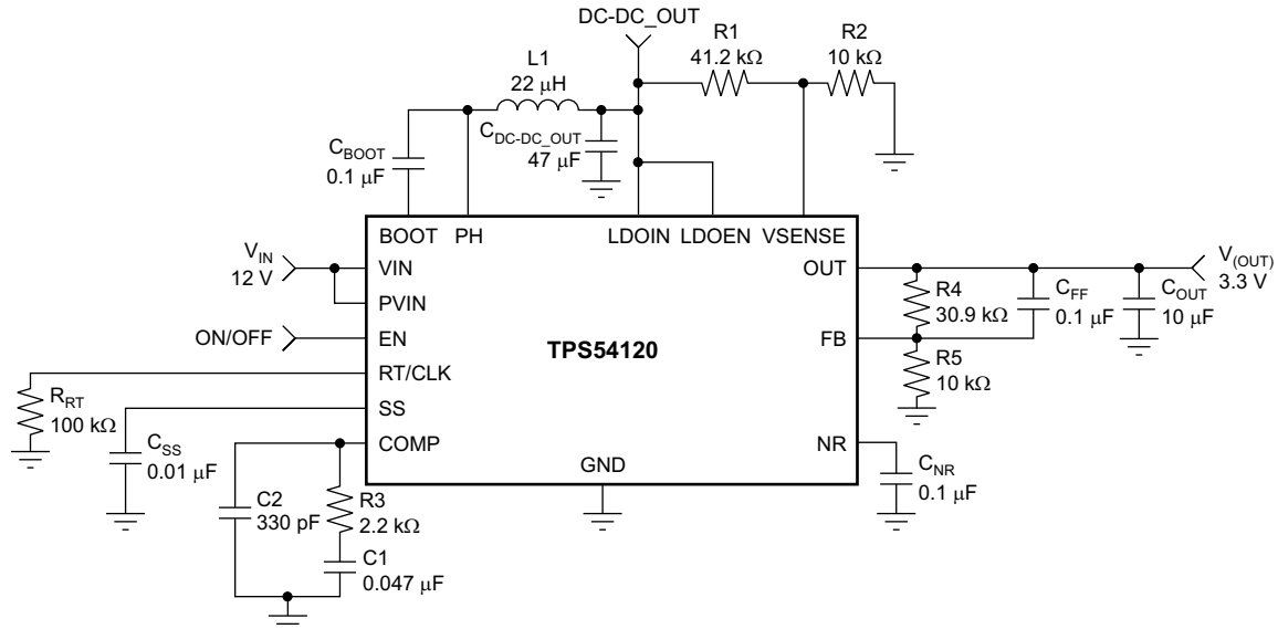
Figure 28. Typical Application
