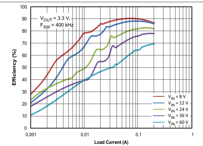
Figure 22. Efficiency vs Output Current
