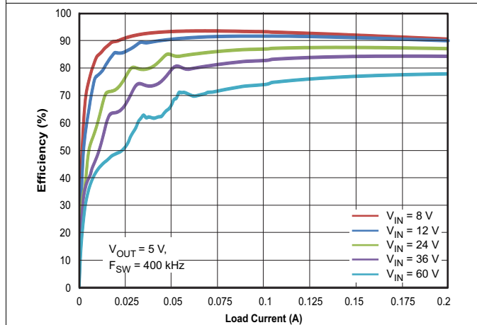
Figure 23. Efficiency vs Output Current
