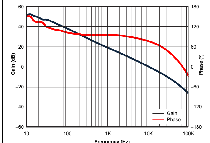
Figure 25. Gain vs Phase
