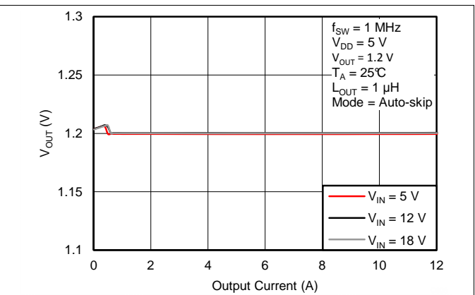
Figure 54. Output Voltage vs. Output Current
