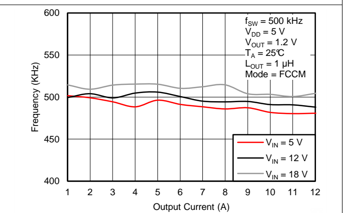
Figure 56. Switching Frequency vs. Output Current
